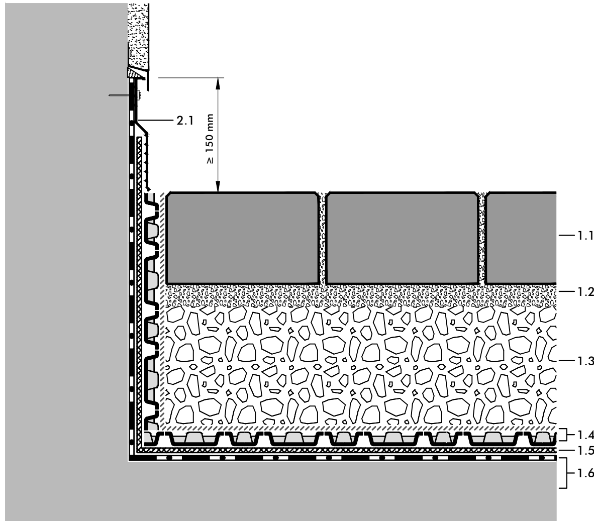
2.1 Clamping and Protection Profile AP 150
